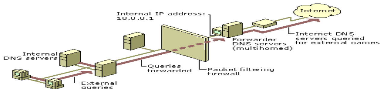
Figure 4.1: external name queries are directed using forwarders.
