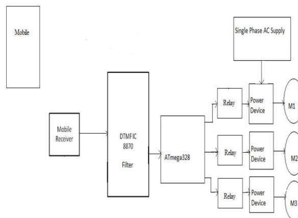
Fig: Block diagram of wireless control of AC motor using DTMF
