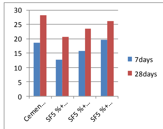
Influence of Silica fume 5% and GGBS 10%, 20%, 30% Development of Compressive Strength of Cement Mortar (1:3)
