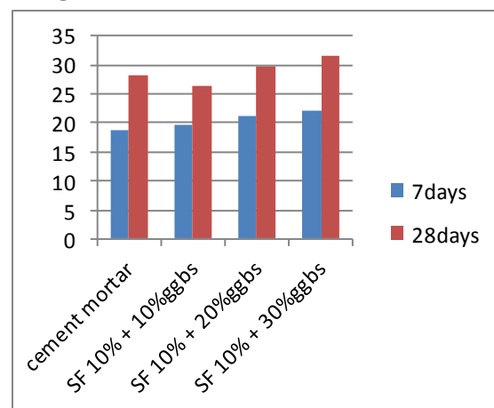
Influence of Silica fume 5% and GGBS 10%, 20%, 30% Development of Compressive Strength of Cement Mortar (1:3)
