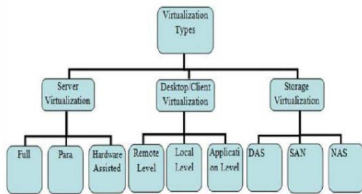
Fig 1 : Virtualization Types
