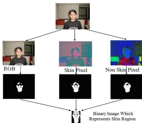
Figure 2. Face Detection Algorithm Flow
